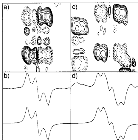
FIGURE 6: Determination of proton-proton coupling constants in d(CGCGT*T*GT*TCGCG). The fine structure of the \omega -scaled DQF-COSY spectrum was examined to extract coupling constants. Positive contours are solid lines, and negative contours are dashed lines. (a) Expansion of the cross peak between the H1' and H2' of G 13 . (b) (Upper trace) Horizontal section through the cross peak in (a); (lower trace) calculated from a nonlinear least-squares fit of a sum of antiphase Lorentzian lines to the cross section. Fitted parameters are J_{H1'-H2'} = 8.4 Hz, J_{H1'-H2''} = 6.0 Hz, width = 3.0 Hz, amplitude = -7.68, and base-line offset = -0.037. (c) Expansion of the cross peak between the H1' and H2' of residues T 5 . An extra coupling is observed in the H1' direction due to coupling with 13 C at the C6 carbon. (d) (Upper trace) Horizontal cross section through the cross peak in (c); (lower trace) calculated from a nonlinear least-squares fit of a sum of antiphase Lorentzian lines to the cross section. Fitted parameters are J_{H1'-H2'} = 7.2 Hz, J_{H1'-H2''} = 6.5 Hz, J_{H1'-C6} = 3.8 Hz, width = 3.1 Hz, amplitude = -4.14, and base-line offset = -0.02.
