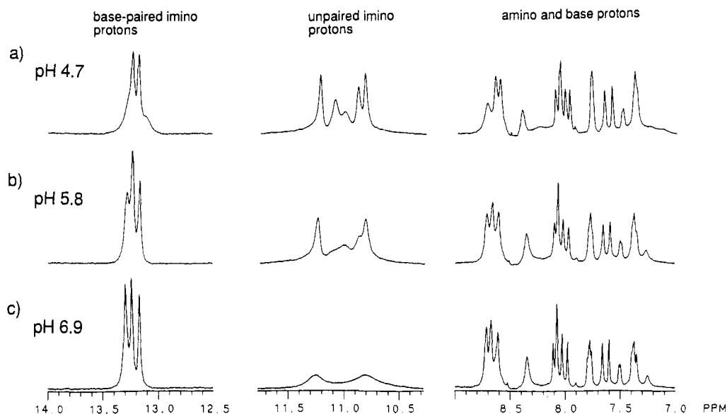
FIGURE 5: 500-MHz NMR spectra of d(CGCGTTGTCGCG) in \text{H}_2\text{O} at 5 °C. Spectra were recorded by using the 1331 pulse sequence with the excitation maximum centered at 11 ppm, as a function of pH: (a) pH 4.7, (b) pH 5.8, and (c) pH 6.9.
