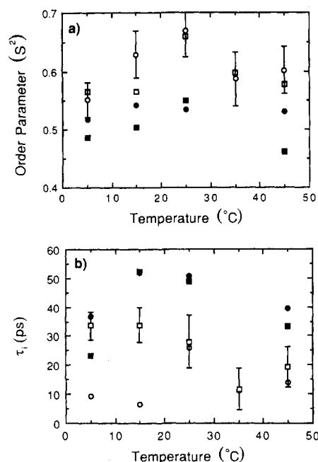
FIGURE 11: (a) Order parameters and (b) internal correlation times for the thymidine C6 carbons: ( \square ) T_9 , ( \blacksquare ) T_8 , ( \bullet ) T_6 , ( \circ ) T_5 . The order parameters and the correlation times for internal motions were obtained from a least-squares fit to the relaxation data. Error bars indicated for the error in the order parameter are for residue T_9 and are the largest errors among the four residues. The errors for residue T_5 are the smallest and are approximately 50% smaller. The errors for the internal correlation time are for residue T_8 and are the largest errors.
