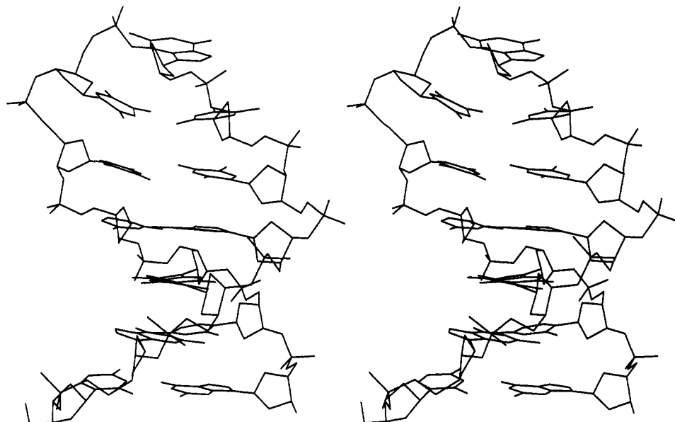
FIGURE 12: Stereo pair diagram of the energy-minimized model of the hairpin formed by d(CGCGTTGTTTCGCG).
