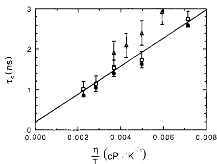
FIGURE 10: Stokes-Einstein plot for the rotational correlation times from three different nuclei: (●) ^1\text{H} , (□) ^{13}\text{C} , (Δ) ^{31}\text{P} . The rotational correlation time was experimentally determined from the cross-relaxation rate between cytosine H5 and H6, from T_1 and NOE measurements on the thymidine C6 carbon, and from T_1 and T_2 measurements on P 5 . Error bars are indicated for the data from phosphorus relaxation, and the error bars on the carbon data points are the errors from the least-squares fit. The line drawn is the least-squares line fit to the correlation time obtained from the carbon data.
