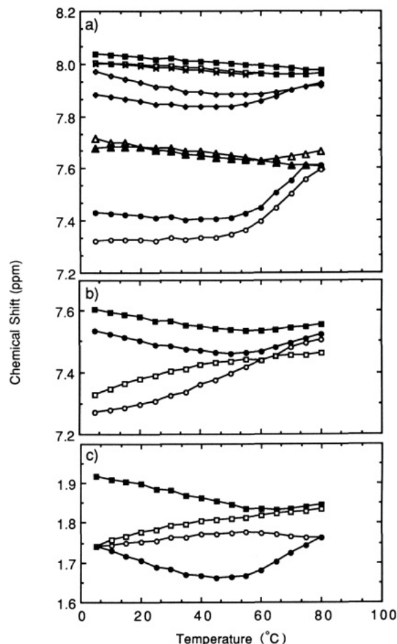
FIGURE 4: Temperature dependence of the chemical shifts of selected protons in d(CGCGTTGTTTCGCG). (a) Guanine H8 protons (■) G 2 , (□) G 11 , (×) G 13 , (◇) G 4 , (◆) G 7 ; cytosine H6 protons (Δ) C 1 , (▲) C 10 , (●) C 12 , (○) C 3 . (b) Thymidine H6 protons. (c) Thymidine methyl protons (■) T 9 , (●) T 8 , (□) T 6 , (○) T 5 .
